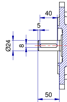
Shaft detail
