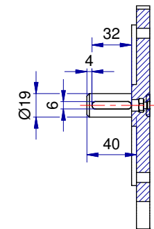
Shaft detail
