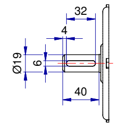
Shaft detail
