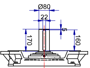
Shaft detail
