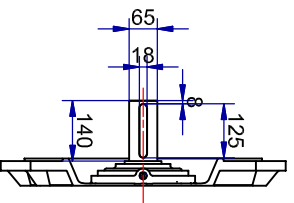
Shaft detail
