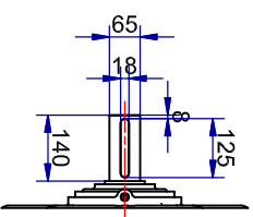
Shaft detail
