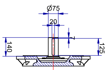
Shaft detail
