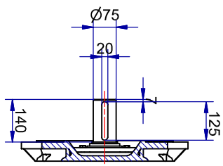
Shaft detail
