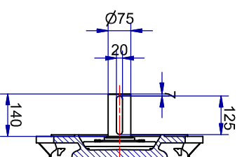
Shaft detail
