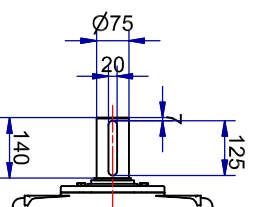
Shaft detail
