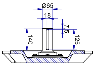
Shaft detail
