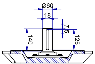
Shaft detail
