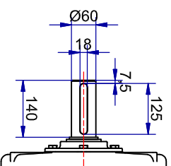
Shaft detail
