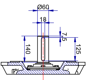
Shaft detail
