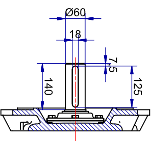
Shaft detail
