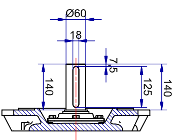
Shaft detail
