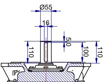
Shaft detail
