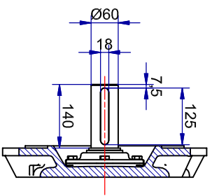
Shaft detail
