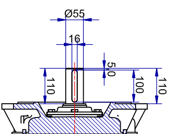
Shaft detail
