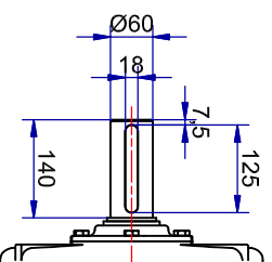
Shaft detail
