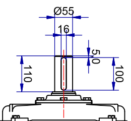
Shaft detail
