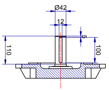
Shaft detail
