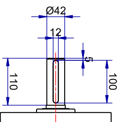
Shaft detail
