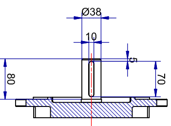
Shaft detail
