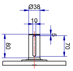
Shaft detail
