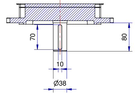
Shaft detail
