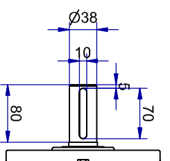
Shaft detail
